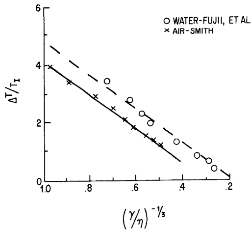
FIG. 6. Plot of temperature data from [1, 2, 5] in inner variables (heat flux version).
