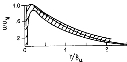
FIG. 8. Plot of velocity from [1, 3] in outer variables (adapted from [3]).
