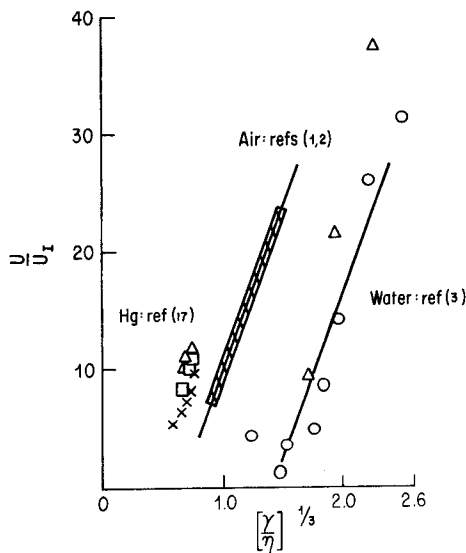
FIG. 7. Plot of velocity data from [2, 3, 17] in inner variables (heat flux version).
