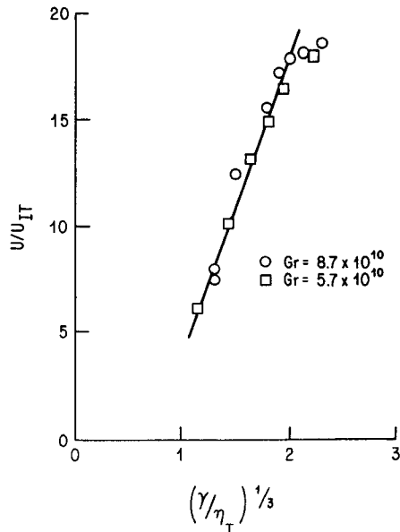
FIG. 5. Plot of velocity data from [2] in inner variables (wall temperature version).
