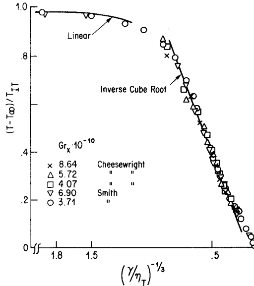
FIG. 4. Plot of temperature data of references [1] and [2] in inner variables (wall temperature version).
