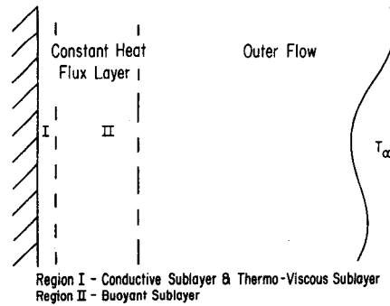
FIG. 2. Diagram showing major regions of the boundary layer. Region I includes conductive and thermo-viscous sublayers. Region II is buoyant sublayer.
