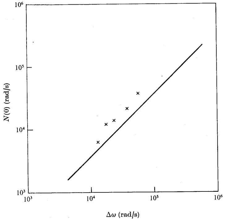
FIGURE 20. Dependence of spectral height N(0) on \Delta\omega = \bar{u}k_* ( k_* calculated from lens focal length). —, N(0) = 0.368\Delta\omega . Uniform laminar flow; \bar{u} = 80 cm/s.
