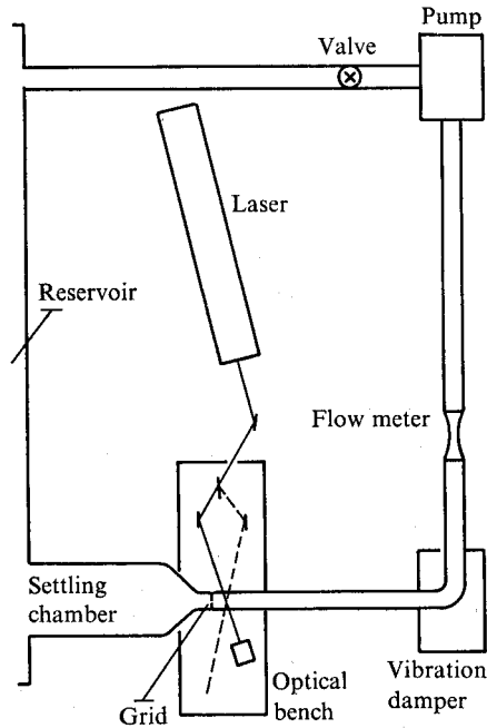
FIGURE 18. Flow facility.
