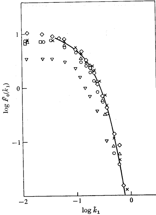
FIGURE 22. Corrected spectra shown with spectrum measured with hot-film anemometer. R_M = uM/\nu = 2 \times 10^3 , \sin \frac{1}{2}\theta = 0.145 .
