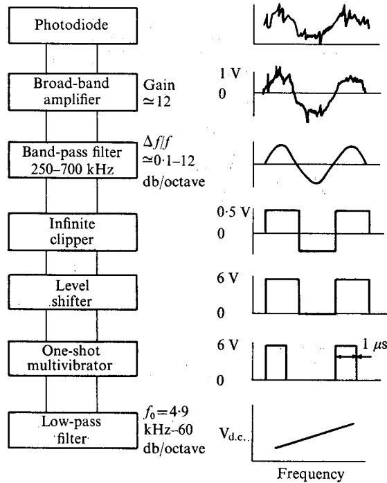
FIGURE 17. Signal processor.
