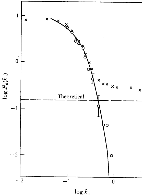
FIGURE 21. Measured (crosses) and corrected (circles) spectra in turbulent flow shown with spectrum measured with hot-film anemometer. R_M = 2 \times 10^3 , x/M = 45 , \tilde{k}_* = 3.9 , \sin \frac{1}{2}\theta = 0.145 .
