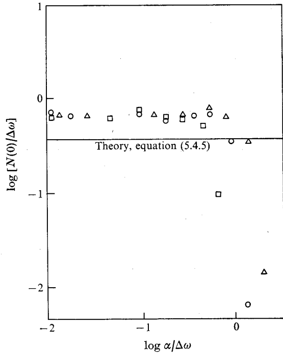
FIGURE 19. Measured ambiguity spectra in laminar flow. \Delta\omega = k_* \bar{u} , \bar{u} = 80 cm/s. \Delta , k_* = 282 cm ^{-1} ; \circ , k_* = 352 cm ^{-1} ; \square , k_* = 470 cm ^{-1} .
