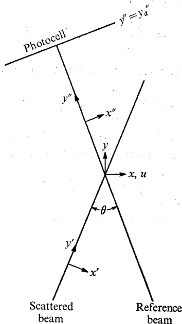
FIGURE 1. Scattering co-ordinates. Origin of all co-ordinate systems is chosen at centre of scattering volume ( z is normal to plane of paper).
