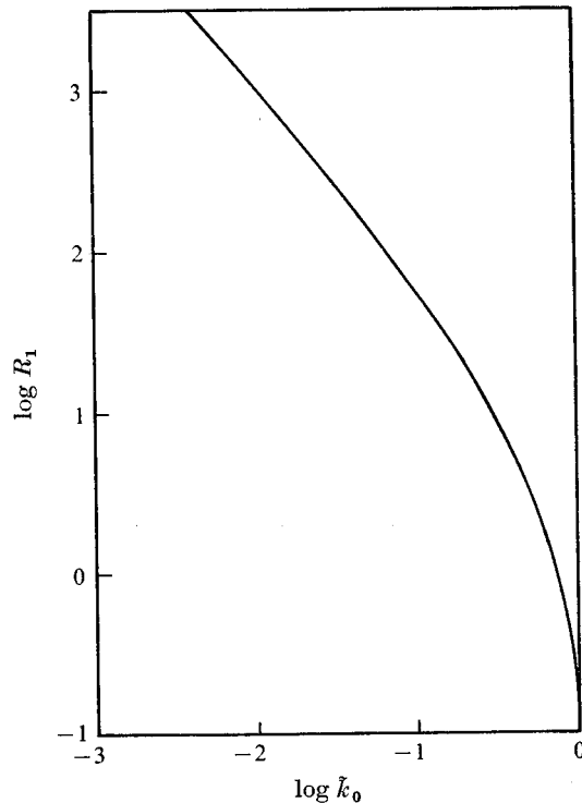
FIGURE 13. Wavenumber corresponding to an ambiguity-to-turbulence ratio of unity under optimum conditions. \bar{F}_{11}^1(k_0) = 1.68 \times 10^{-2} R_1^{\frac{3}{2}} , R = \bar{u}\lambda/2\nu \sin \frac{1}{2}\theta = 2\pi\bar{u}^2/\nu\bar{\omega}_0 , R_1 = R/\sin^{\frac{1}{2}} \frac{1}{2}\theta .
