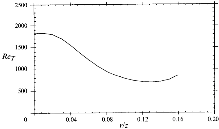
FIGURE 15. Profile of the turbulence Reynolds number across the plume at a vertical distance of z/D = 15.7 .
