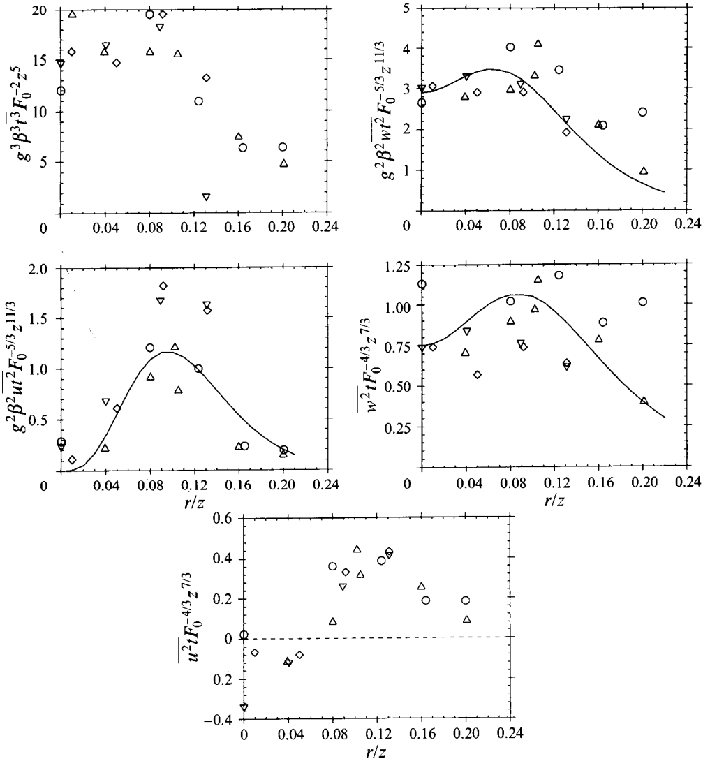
FIGURE 8. Profiles of third moments involving temperature plotted in similarity variables. For meaning of symbols see caption of figure 5(a).
