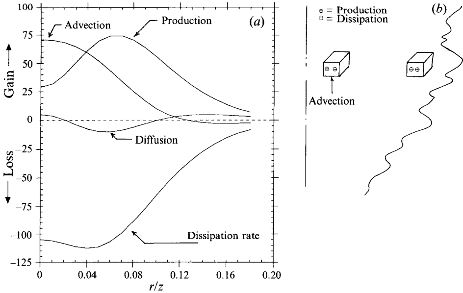
FIGURE 13. (a) Balance of the temperature variance, \frac{1}{2} \overline{t^2} , equation. (b) Sketch showing the different zones of the plume based on the temperature variance balance.
