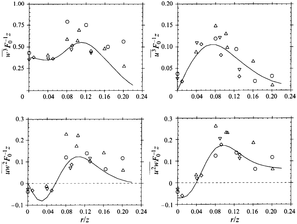
FIGURE 9. Profiles of third moments involving velocity only plotted in similarity variables. For meaning of symbols see caption of figure 5(a).
