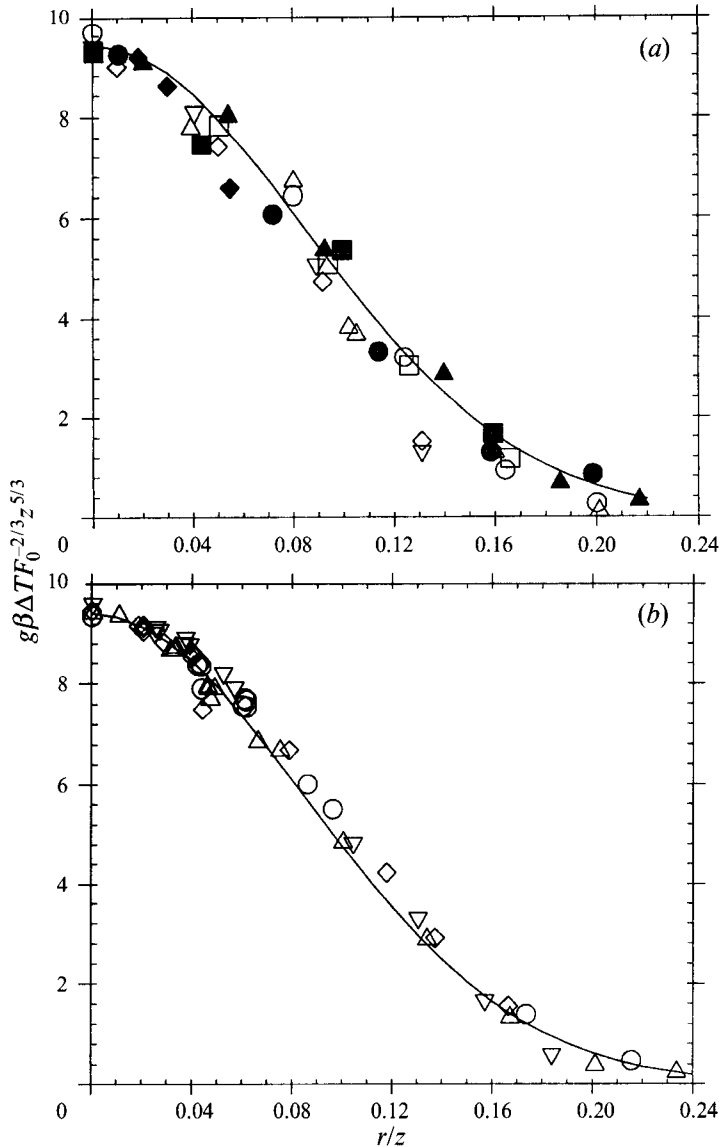
FIGURE 5. (a) Profile of mean buoyancy in similarity variables. Solid symbols refer to the two-wire probe measurements and open symbols refer to the three-wire probe measurements. ■, z/D = 11.81 ; ●, z/D = 13.7 ; ▲, z/D = 16.77 ; ◆, z/D = 19.5 ; □, z/D = 10.55 ; ○, z/D = 14 ; △, z/D = 17.3 ; ▽, z/D = 20.31 ; ◇, z/D = 23.46 . (b) Profile of mean buoyancy in similarity variables, as measured with thermocouples. ◇, z/D = 10 ; ○, z/D = 14 ; △, z/D = 19 ; ▽, z/D = 25 .
