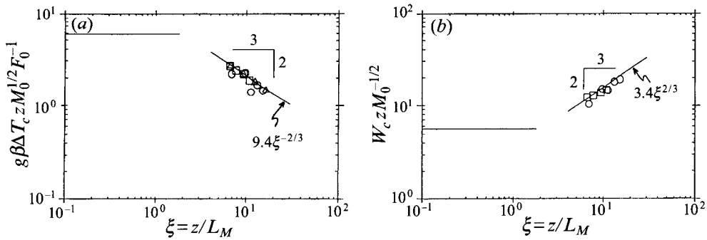
FIGURE 3. (a) Normalized mean buoyancy and (b) normalized mean vertical velocity, along the centreline of the buoyant plume plotted as a function of the normalized vertical distance z/L_M : \triangle , thermocouple data; \square , two-wire probe data; \circ , three-wire probe data.
