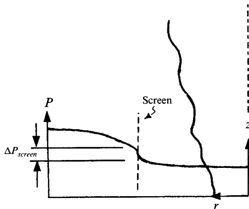
FIGURE 16. Sketch of the radial distribution of pressure near the plume source with a screen placed around its source.
